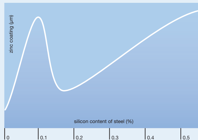
Fig. 5. Approximate thickness of the zinc coating in relation to the silicon (Si) content of the steel.
