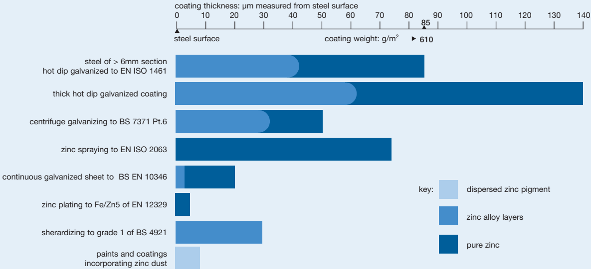
Fig. 9. Zinc coatings compared in terms of coating thickness
