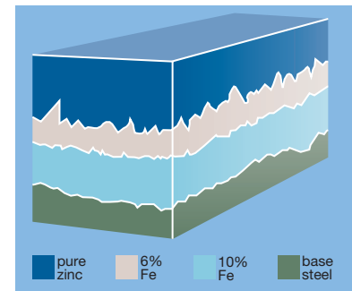
Schematic section through a typical hot dip galvanized coating.
